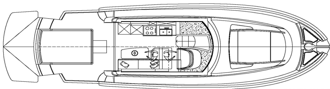
MAIN DECK
